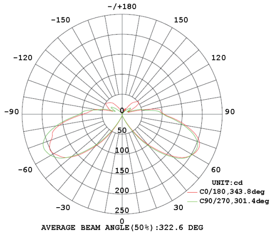
INTENSITY DISTRIBUTION DIAGRAM IN C PLANS
